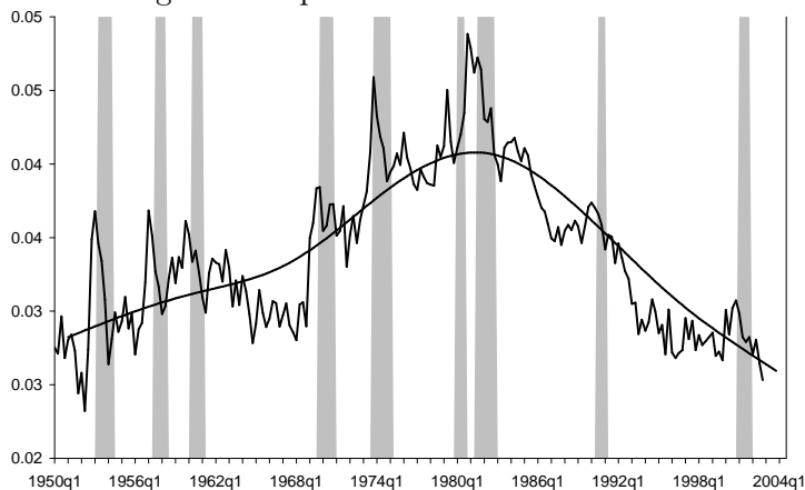
Figure 9: Separation rate - Shimer data
