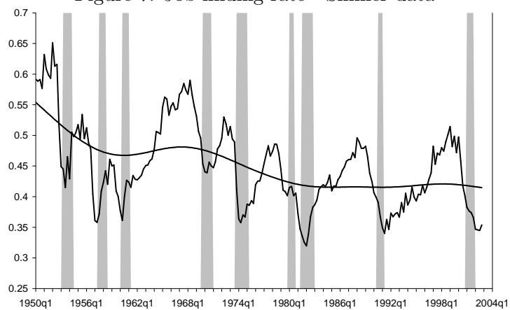
Figure 7: Job finding rate - Shimer data
