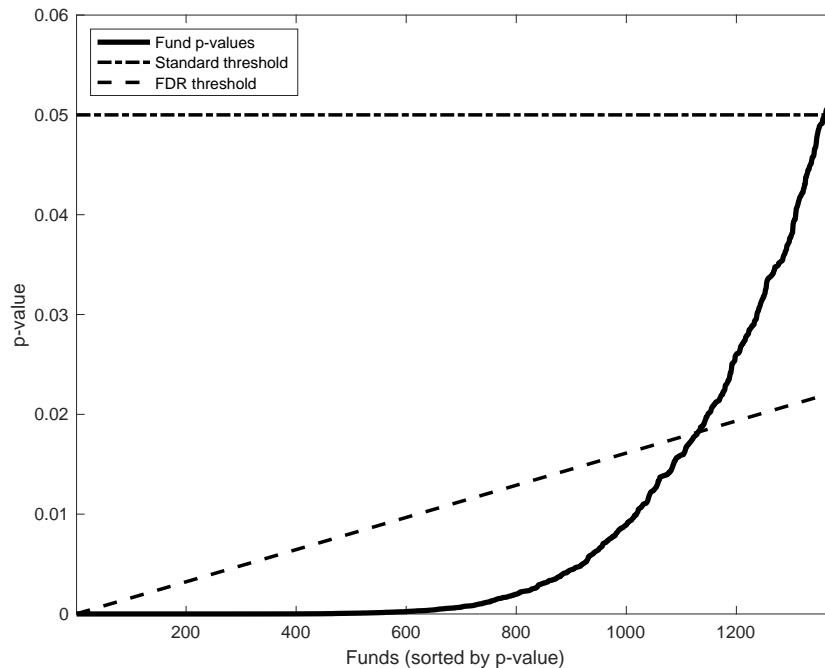
Figure 4: Standard vs. FDR threshold
