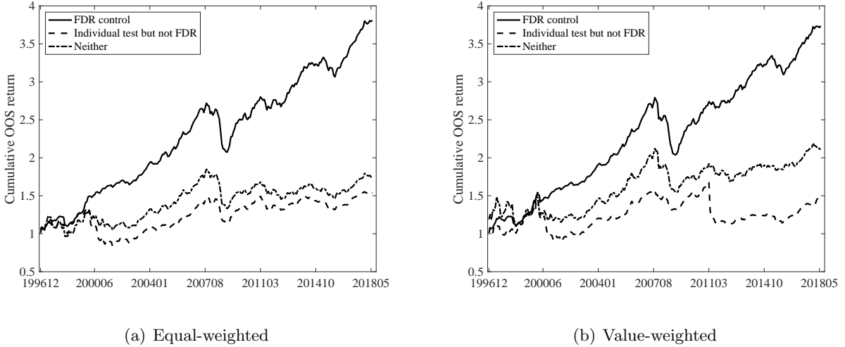
Figure 5: Out-of-sample cumulative portfolio return
